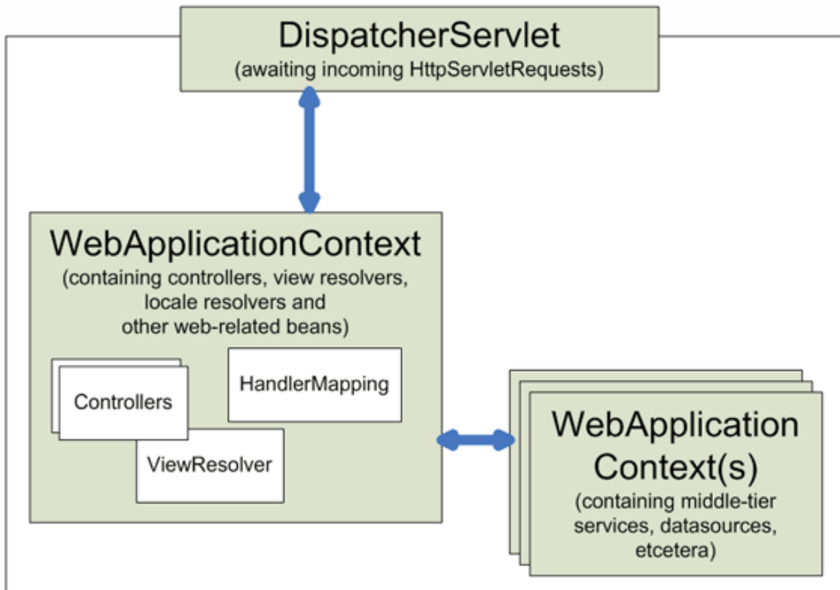
Context hierarchy in Spring Web MVC
